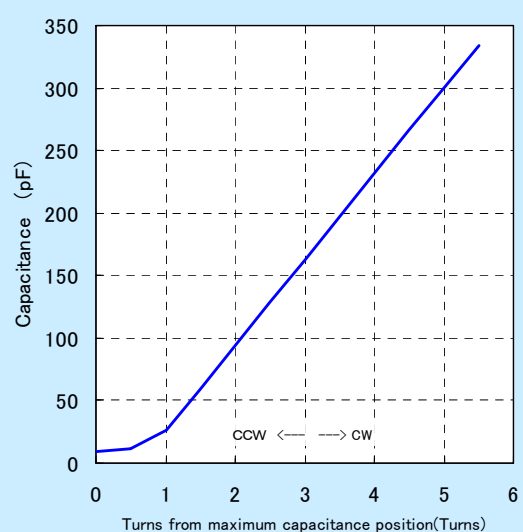
Tuner Turns - Capacitance response
